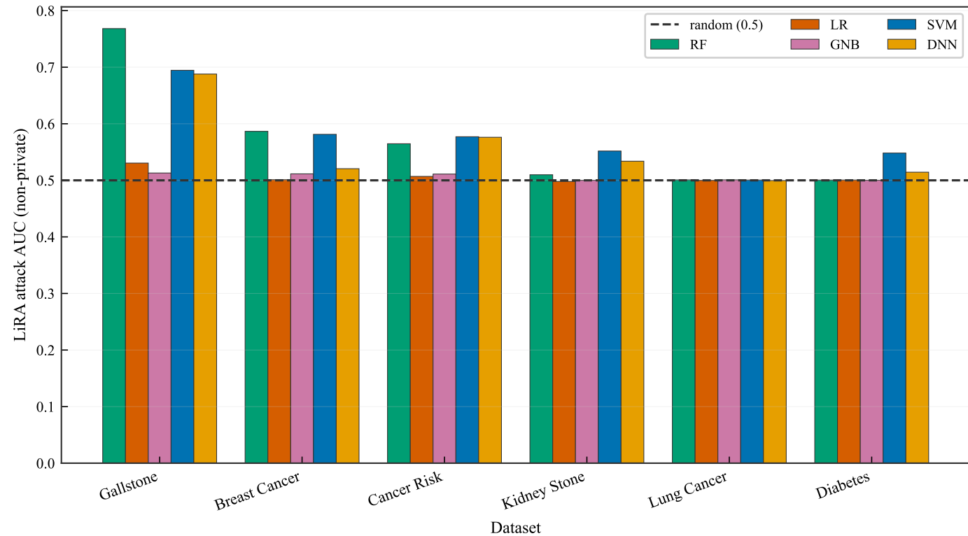
Baseline worst-case leakage (LiRA AUC)
