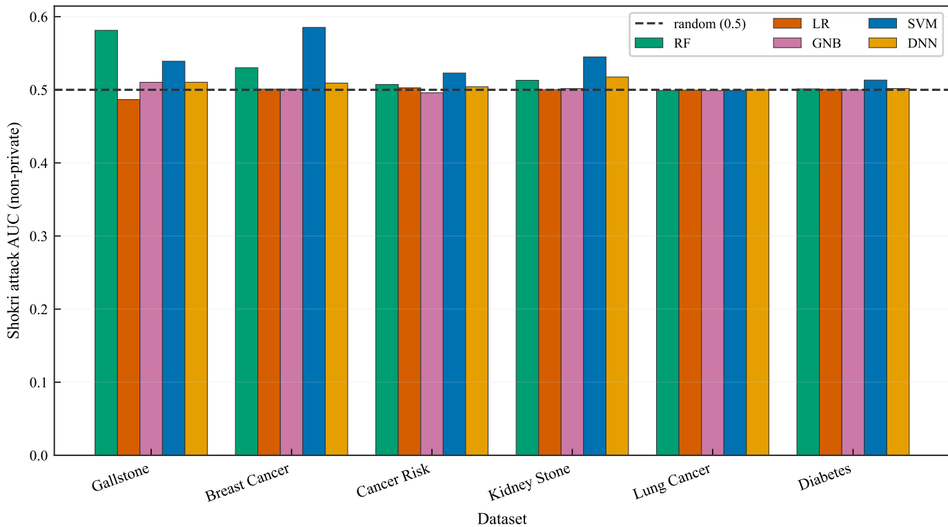
Baseline average-case leakage (Shokri AUC)
