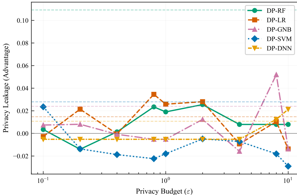
Privacy Leakage — Breast Cancer ( N=569 )
