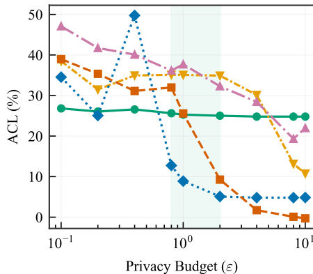
Lung Cancer ( N=50,000 , F=23 )
