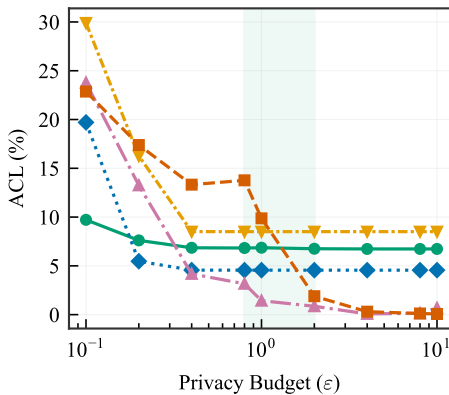
Kidney Stone ( N=4,000 , F=23 )
