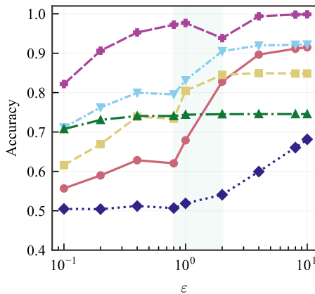
DNN
