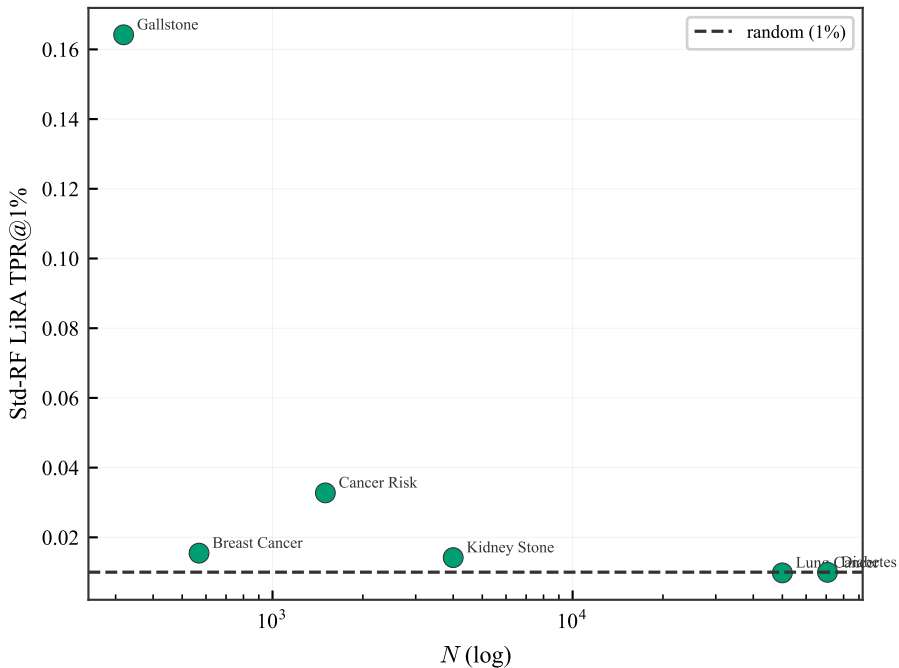
Dataset size vs baseline leakage ( \rho=-0.89 , n=6 )
