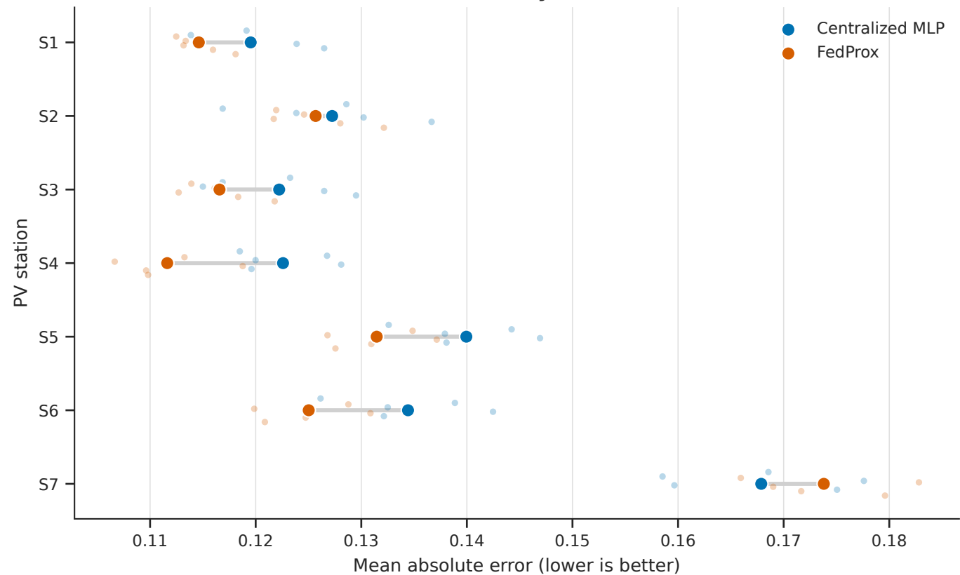
Test MAE by client
