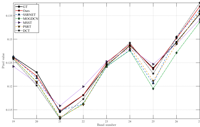
Fig. 8. Spectral response at location (94, 30) in the first test image of the CAVE dataset.
