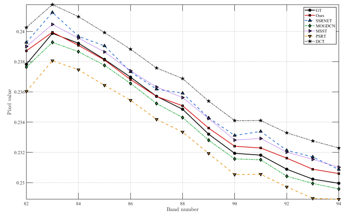
Fig. 9. Spectral response at location (35, 27) in the Chikusei test image.
