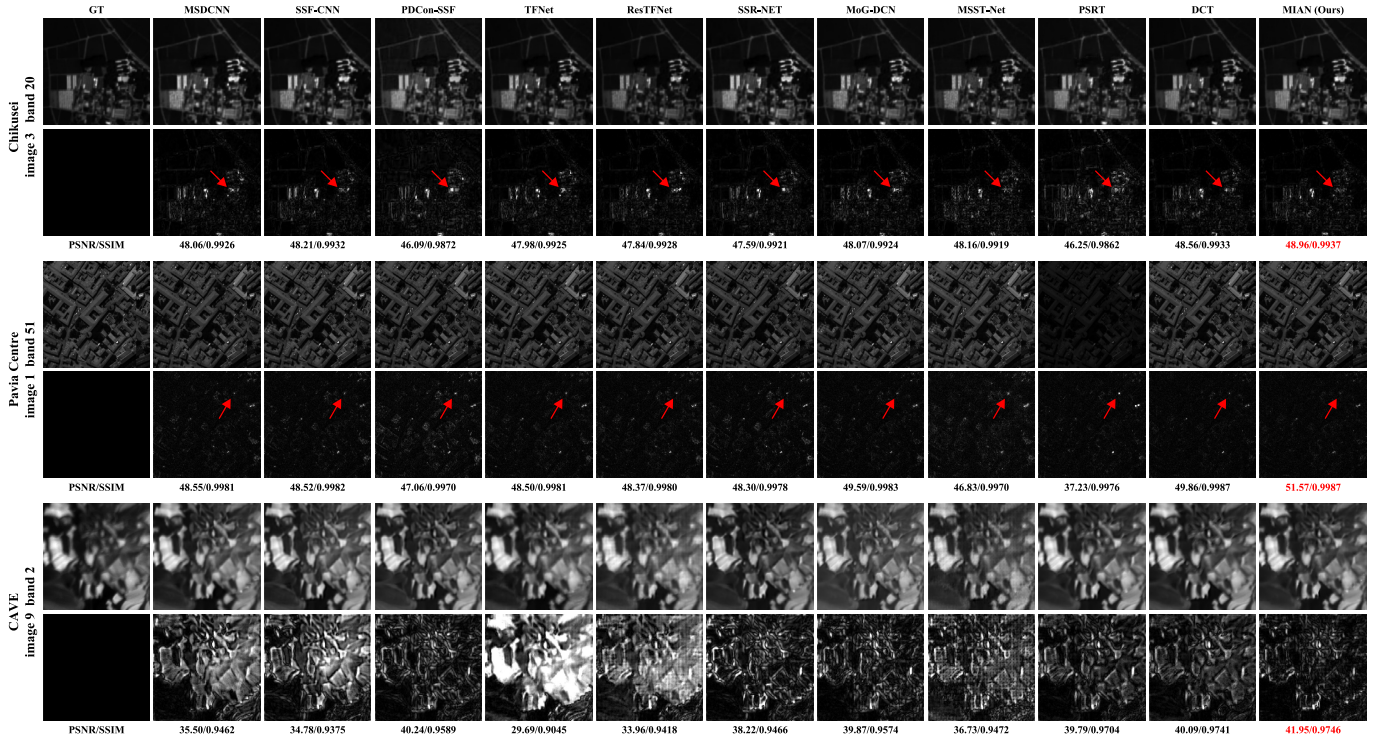
Fig. 6. Reconstructed single-band images and their corresponding error maps for selected bands from the Chikusei, Pavia Centre, and CAVE test sets at \times 4 scale.
