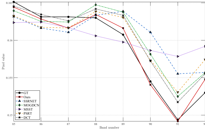
Fig. 10. Spectral response at location (144, 253) in the Pavia Centre test image.
