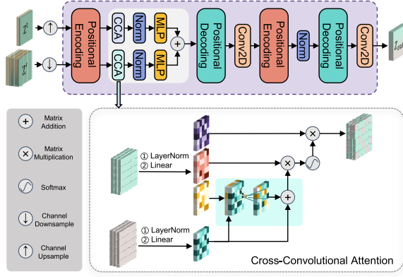
Fig. 3. Structure of MCST.
