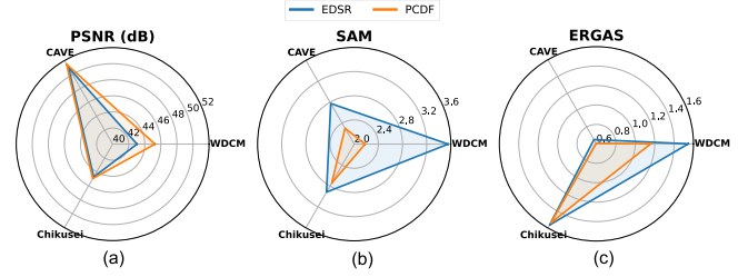
Fig. 9. Ablation experimental results of the CRPF module. Three graphs represent (a) PSNR, (b) SAM, and (c) ERGAS scores of the model on CAVE, WDCM, and Chikusei datasets.
