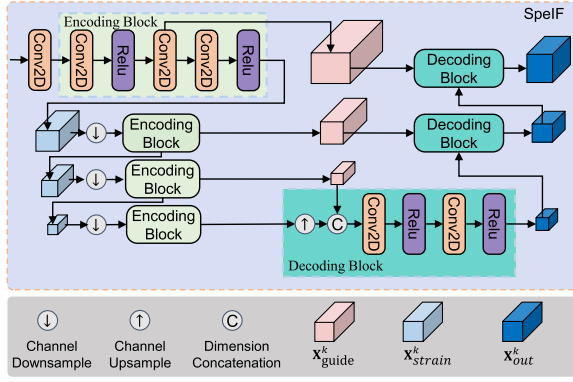
Fig. 2. Structure of SpeIF submodule.
