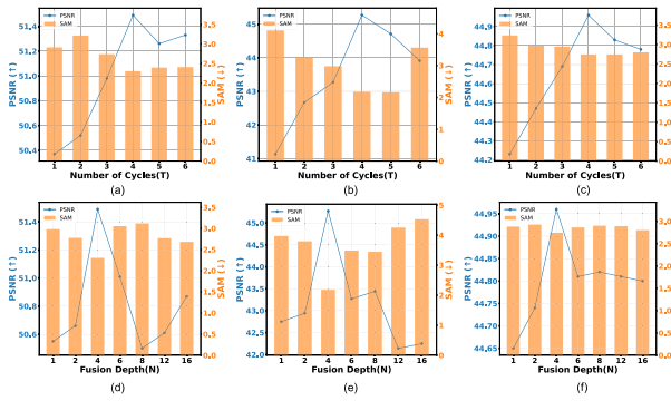
Fig. 10. Parameter analysis of the cycle number T and the fusion depth N on three datasets: (a) CAVE- T , (b) WDCM- T , (c) Chikusei- T , (d) CAVE- N , (e) WDCM- N , and (f) Chikusei- N .
