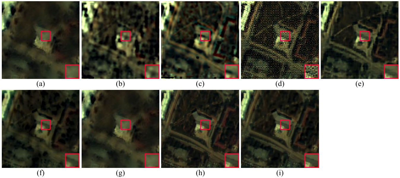
Fig. 8. Fusion images of the pseudo-color composite of the Houston dataset (20th, 10th, and 5th bands). The fusion is performed using (a) EXP, (b) HySure, (c) FUSE, (d) D-UNet, (e) PSRT, (f) HyperPNN, (g) DRCNN, (h) HMPNet, and (i) DIM-HMPF methods.
