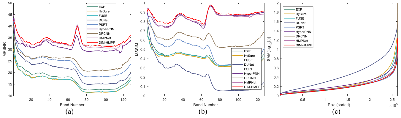
Fig. 7. Different methods were compared on the Chikusei dataset, including (a) corresponding curves of MPSNR, (b) MSSIM, and (c) SAM.
