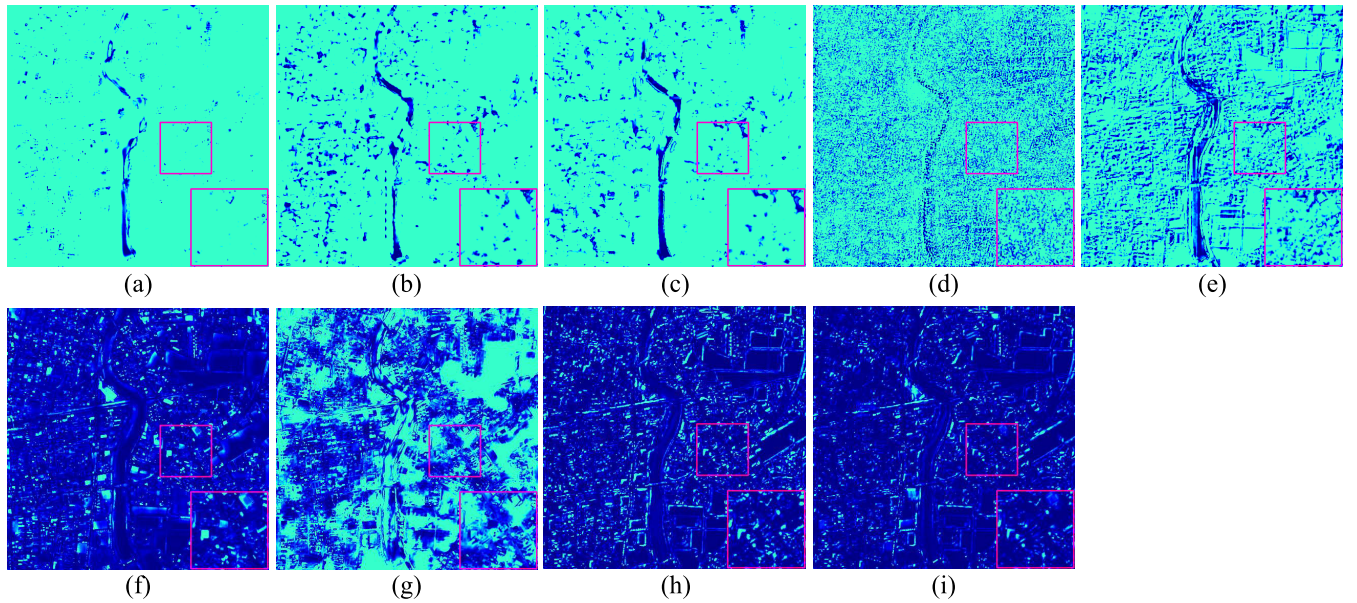
Fig. 6. Error images of the fusion of the Chikusei dataset. The fusion is performed using (a) EXP, (b) HySure, (c) FUSE, (d) D-UNet, (e) PSRT, (f) HyperPNN, (g) DRCNN, (h) HMPNet, and (i) DIM-HMPF methods.
