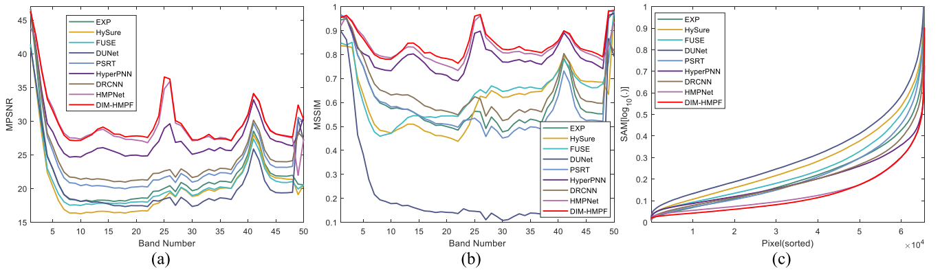
Fig. 10. Different methods were compared on the Houston dataset, including (a) corresponding curves of MPSNR, (b) MSSIM, and (c) SAM.
