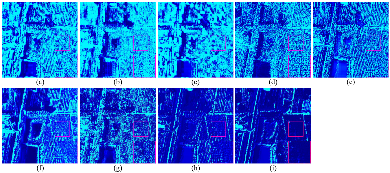
Fig. 12. Error images of the fusion of the Xiongan dataset. The fusion is performed using (a) EXP, (b) HySure, (c) FUSE, (d) D-UNet, (e) PSRT, (f) HyperPNN, (g) DRCNN, (h) HMPNet, and (i) DIM-HMPF methods.
