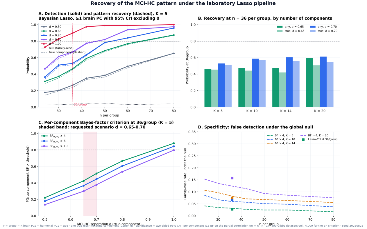
Figure 9: Fixed-design addendum. (A) Detection (solid) and pattern recovery (dashed) as a function of n per group at K = 5 ; the dotted red line marks 36 per group. (B) Both probabilities at 36 per group across K . (C) The per-component Bayes-factor criterion at the focal point; the shaded band is d = 0.65-0.70 . (D) Specificity under the global null.
