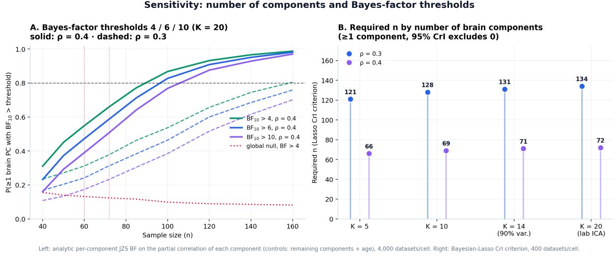
Figure 6: Sensitivity analyses. (A) Probability that at least one brain component reaches \text{BF}_{H_1/H_0} > u for u = 4, 6, 10 ( K = 20 ; solid \rho = 0.4 , dashed \rho = 0.3 ; red dotted line = global null at \text{BF} > 4 ). (B) Required n under the Lasso-CrI criterion as a function of the number of retained components K .
