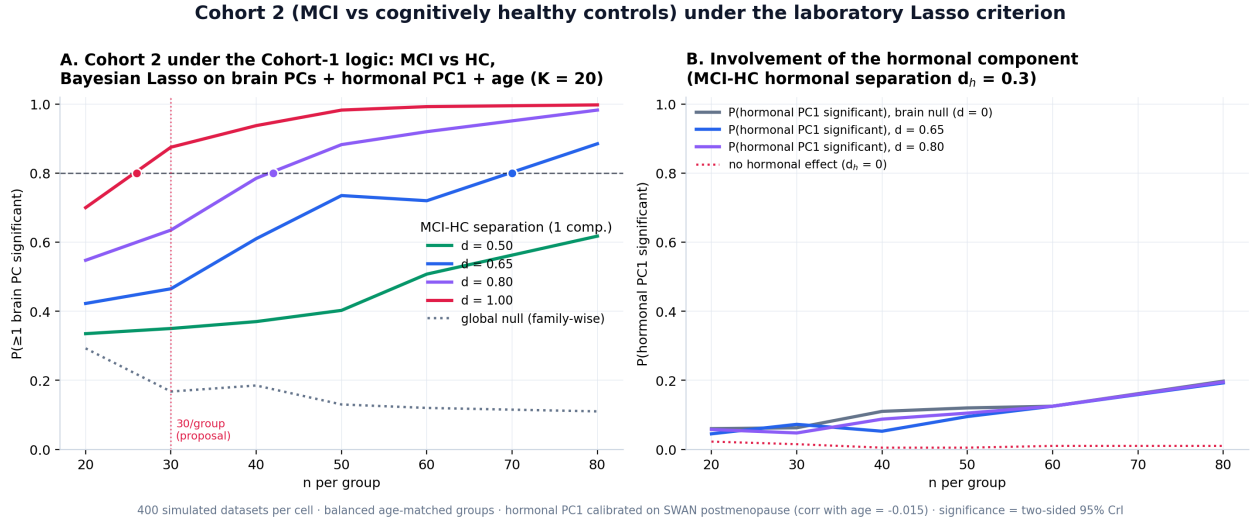
Figure 8: Cohort 2 under the laboratory Lasso criterion. (A) Probability that at least one brain component separates MCI from HC (95% CrI, two-sided) as a function of n per group; dots mark the required n ; the grey dotted line is the family-wise rate under the global null. (B) Probability that the hormonal PC1 coefficient is significant when the true MCI–HC hormonal separation is d_h = 0.3 (red dotted line: d_h = 0 ).
