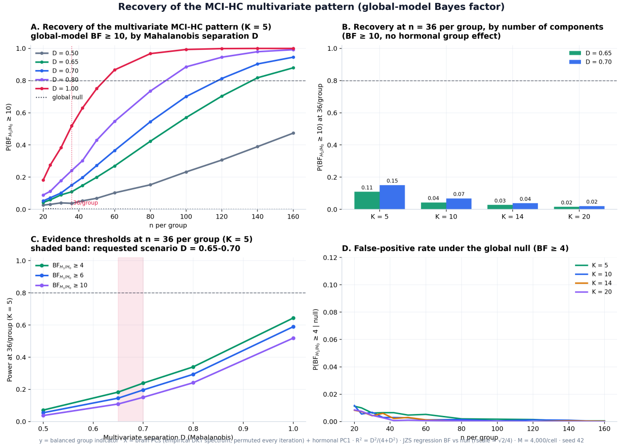
Figure 4: Fixed-design addendum. (A) Recovery as a function of n per group at K = 5 and \text{BF}_{H_1/H_0} \geq 10 , by separation D . (B) Recovery at 36 per group across K . (C) Evidence thresholds at the focal point; the shaded band is D = 0.65 – 0.70 . (D) False-positive rate under the global null.
