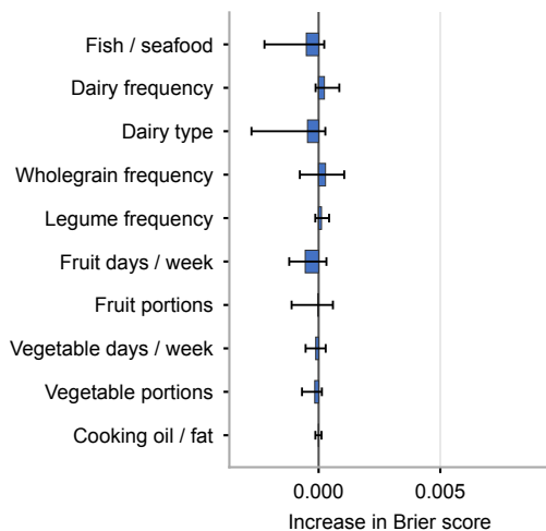
c Random forest
