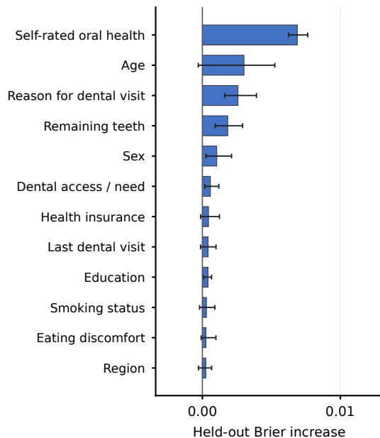
b Random forest
