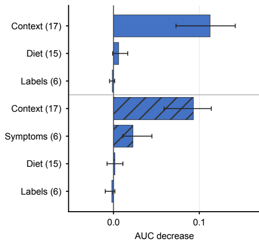
c Spline logistic / AUC
