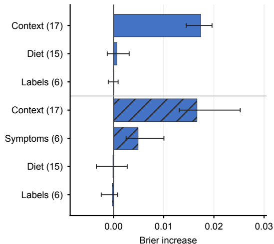
a Spline logistic / Brier
