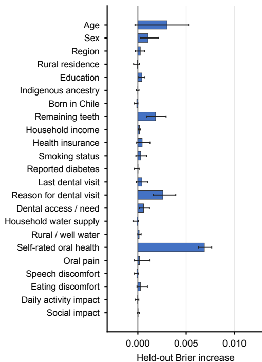
c Random forest Non-dietary information
