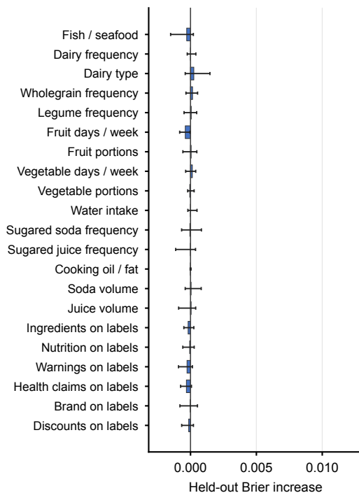
d Random forest Diet and label behaviours
