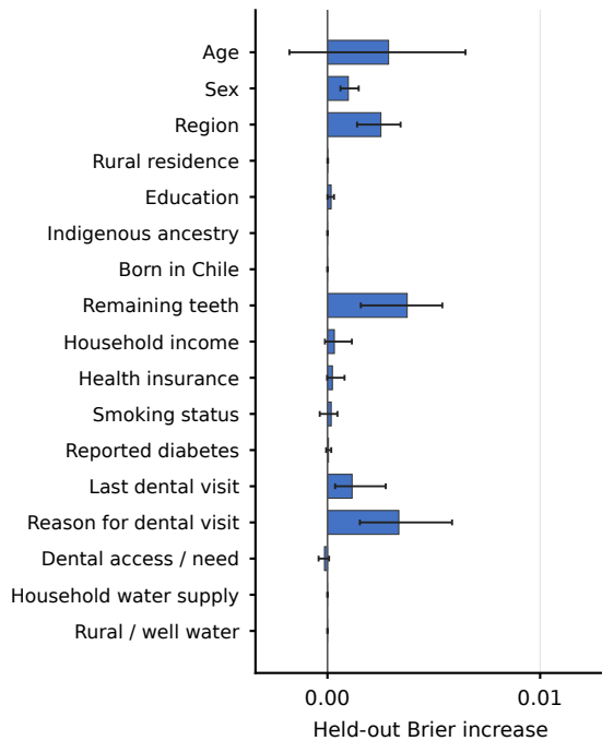
c Gradient boosting
