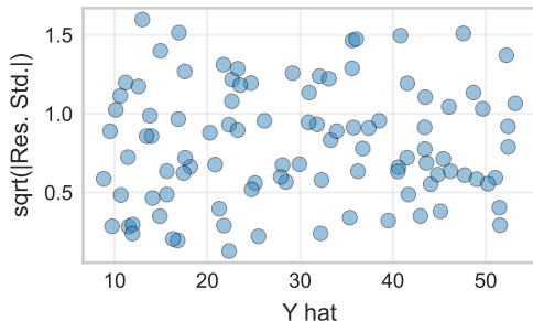
Scale-Location
