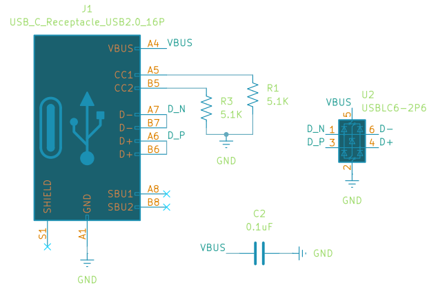
USB-C + ESD protection
