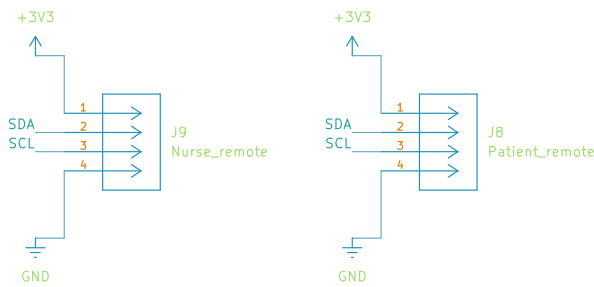
Patient and Nurse Remote Connection points
