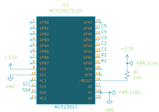
MCP23017 I/O expander
