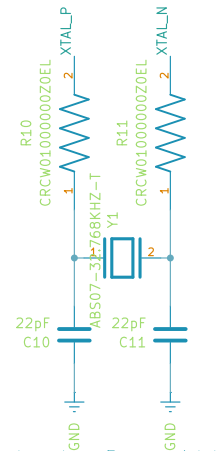
Crystal Oscillator
