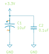
Power Filter Circuit
