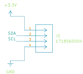
Connection point to Controller
