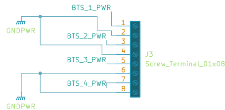
BTS Driver Module Motor Power Terminal
