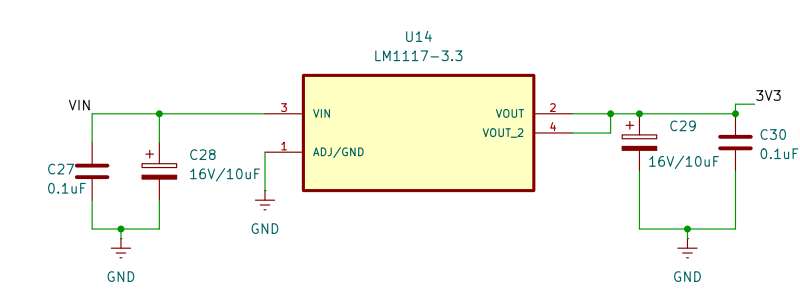
MCU Power Supply
