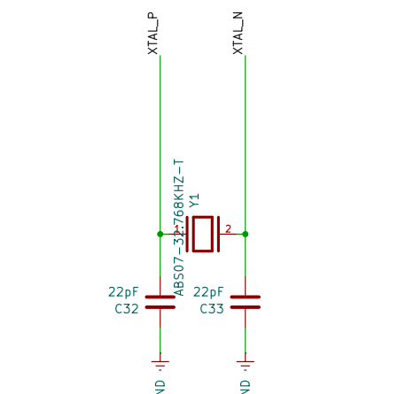
Crystal Oscillator
