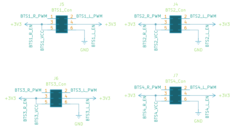
BTS Driver Module Signal Pins Connection point for BTS to Controller
