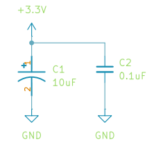
Power Filter Circuit
