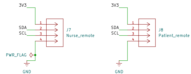
Patient and Nurse Remote Connection points
