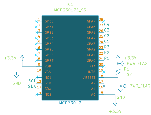
MCP23017 I/O expander
