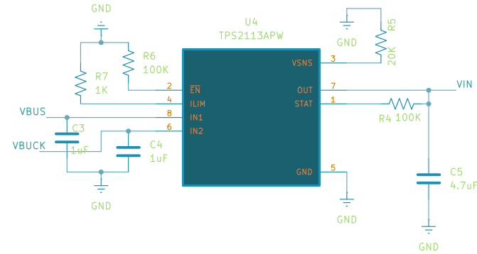
Power MUX selector
