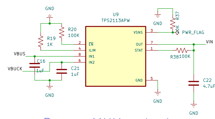
Power MUX selector
