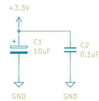
Power Filter Circuit
