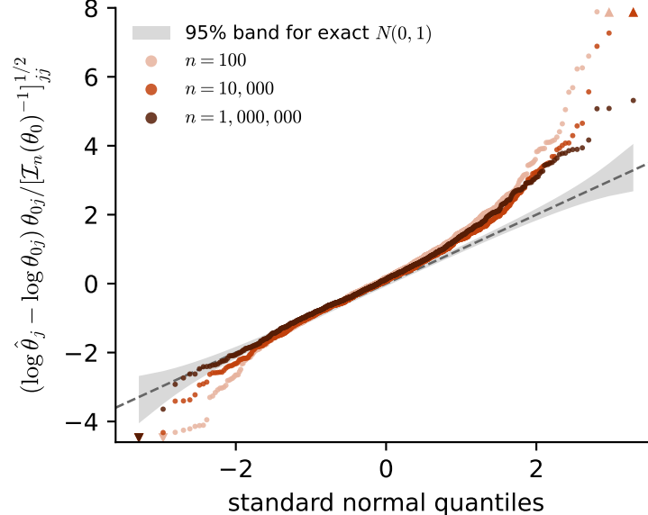
(e) normal Q-Q, \log \ell
