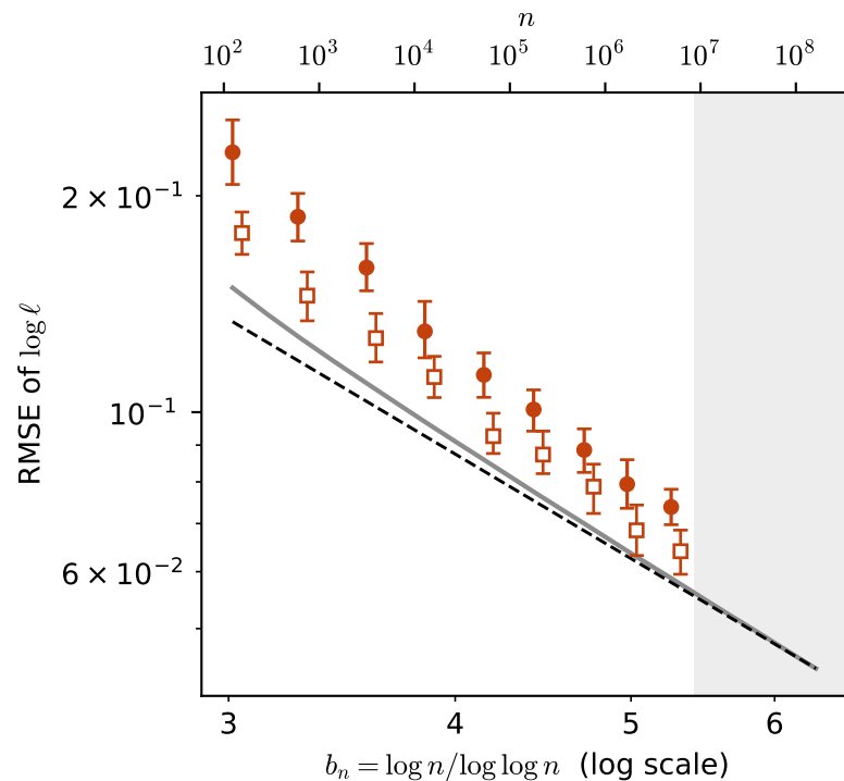
(b) \log \ell
