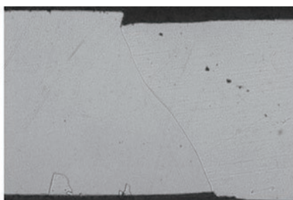
Micrograph of standard Pt wire after 6 hours at 1400 °C under a tensile stress of 2.76 Mpa, showing a large grain structure and resulting grain boundary movement.
