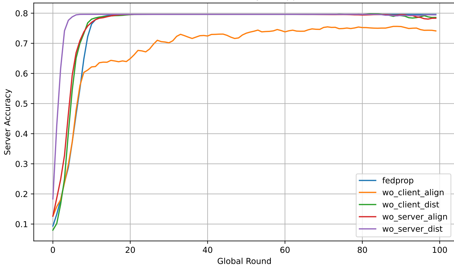
Ablation Study on opp
