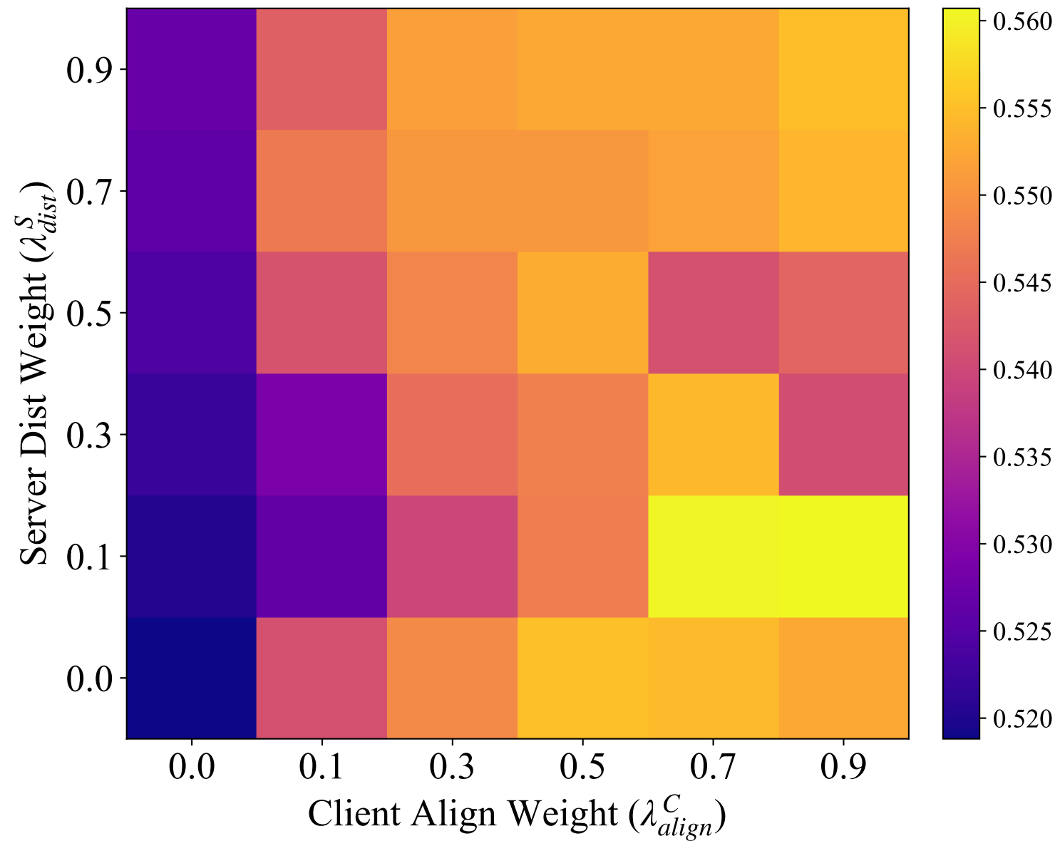
Avg. Client Accuracy Heatmap
