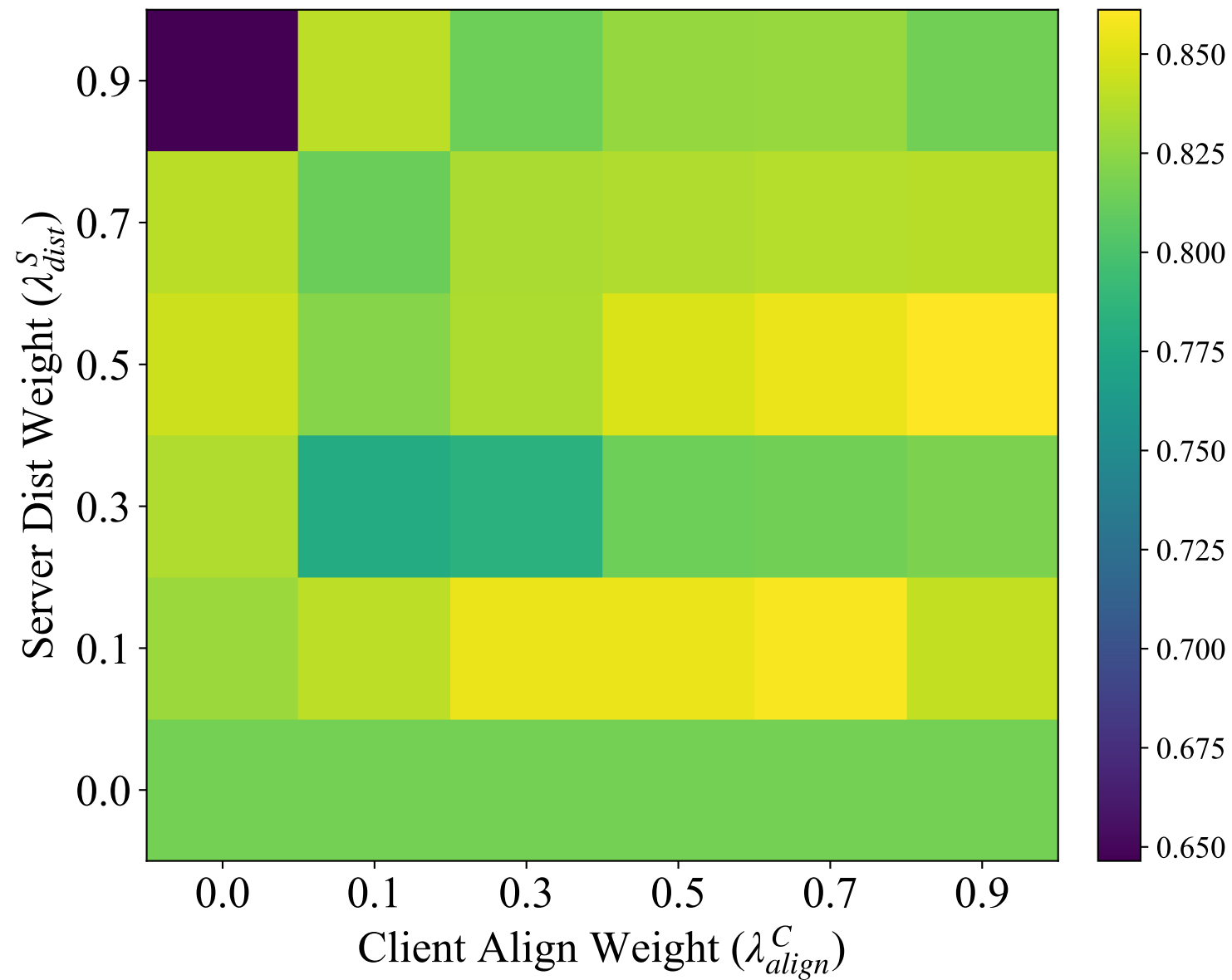
Server Accuracy Heatmap
