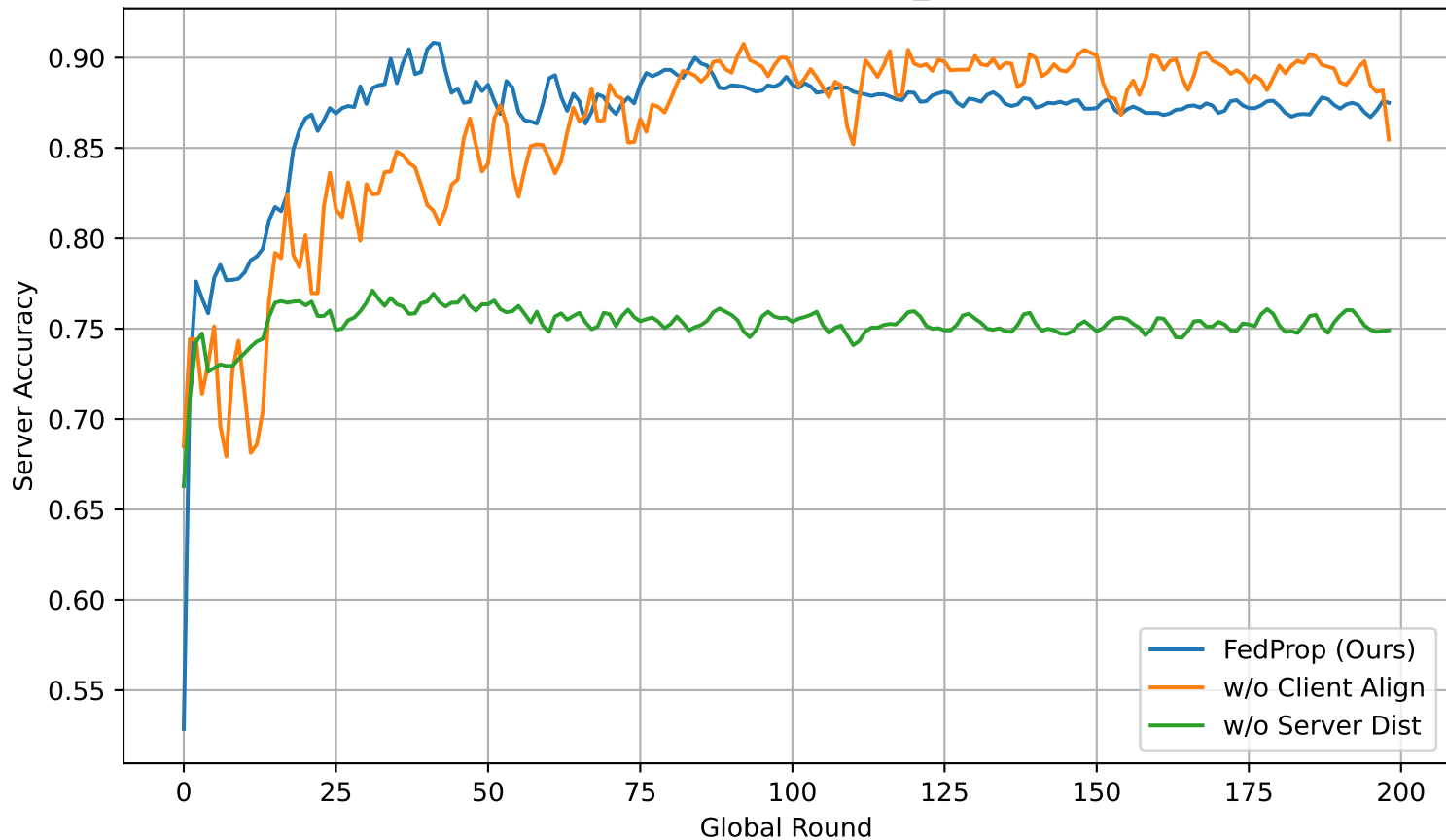
ablation Study on ur_fall
