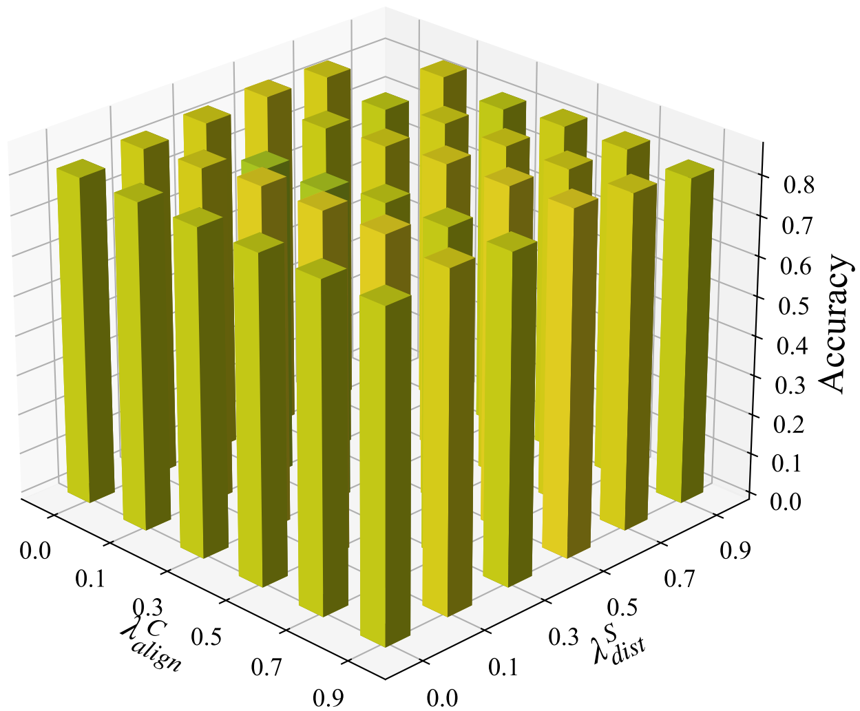
Server Accuracy
