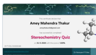
Stereochemistry Quiz
