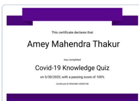
Covid-19 Quiz
