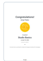
Studio Basics
