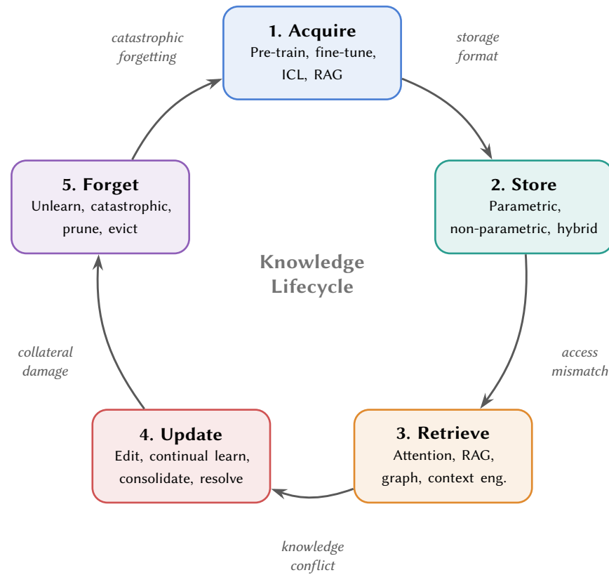
Fig. 1. The Knowledge Lifecycle framework. Knowledge moves clockwise through five stages, each studied by a distinct research community. The italic label on each boundary names what goes wrong when two adjacent stages disagree, following the cross-stage dependencies of §3: acquisition dictates storage format, retrieval must match that format, a fact edited in one store but not the other produces a knowledge conflict, every edit is a small forgetting event with collateral damage, and forgetting feeds back into acquisition as catastrophic forgetting. The stages are well covered in isolation; the five boundaries between them are where the open problems lie, and the failure measured in §8.6 sits on the Retrieve–Update boundary.
