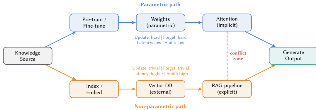
Fig. 2. Two paths through the knowledge lifecycle. The parametric path (top, blue) bakes knowledge into weights during training; it is fast at inference but hard to update or forget. The non-parametric path (bottom, orange) stores knowledge externally; it is easy to modify but depends on retrieval quality. When both paths are active, the “conflict zone” (dashed red) produces the knowledge conflict problem discussed in §5.
