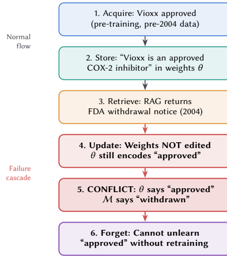
Fig. 3. A lifecycle failure cascade applied to the Rofecoxib (Vioxx) withdrawal. The parametric weights encode an outdated drug approval from pre-training data (Stages 1–2). The RAG index is updated with the FDA withdrawal notice (Stage 3), but no weight edit is applied (Stage 4). The resulting conflict produces a dangerous output (Stage 5), and cannot be resolved without costly retraining (Stage 6). No single-stage benchmark detects this failure.
