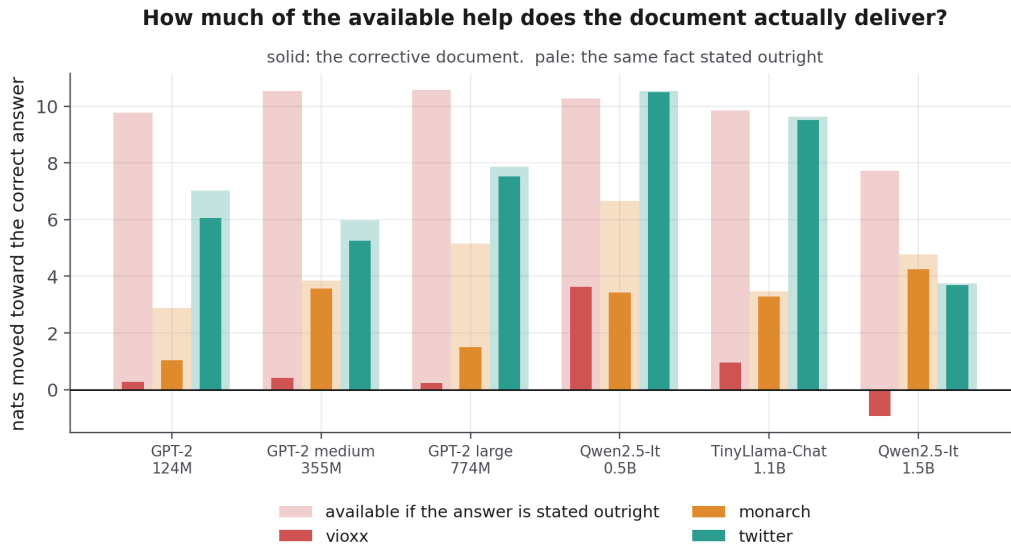
Fig. 6. How much of the available help the corrective document delivers. The pale bar is the surprisal reduction available when the answer is stated outright; the solid bar is what the corrective document achieves. On the Twitter probe the document delivers nearly all of what is available. On Vioxx it delivers almost none of roughly ten nats, and for the largest model it moves the correct answer the wrong way.
