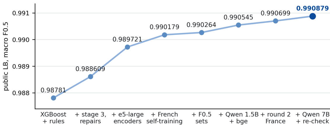
Figure 2. Public leaderboard score after each step. The last point is the submission in this package.
