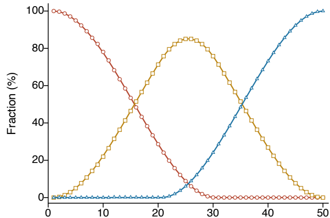
b LCF (known references)
