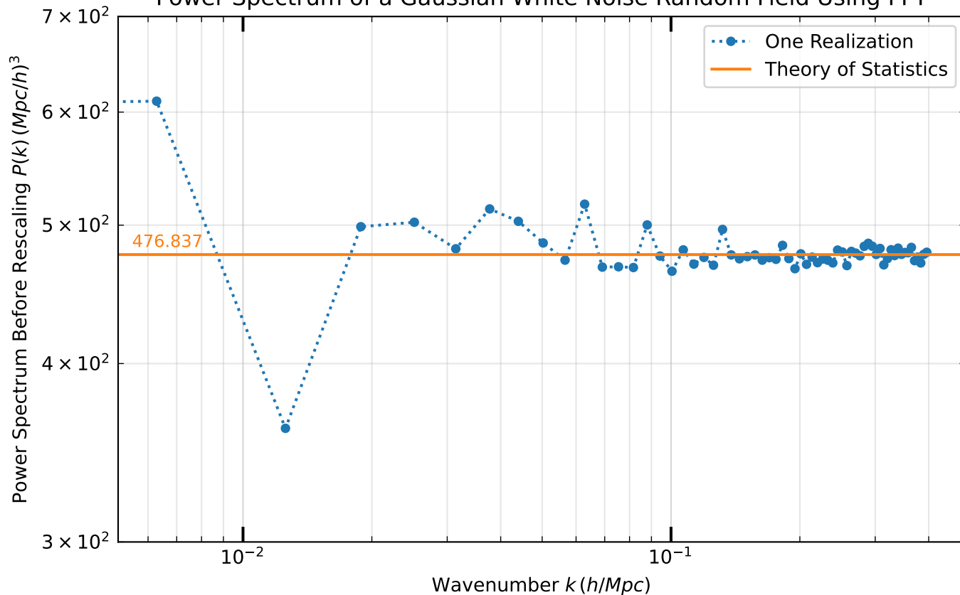
Power Spectrum of a Gaussian White Noise Random Field Using FFT
