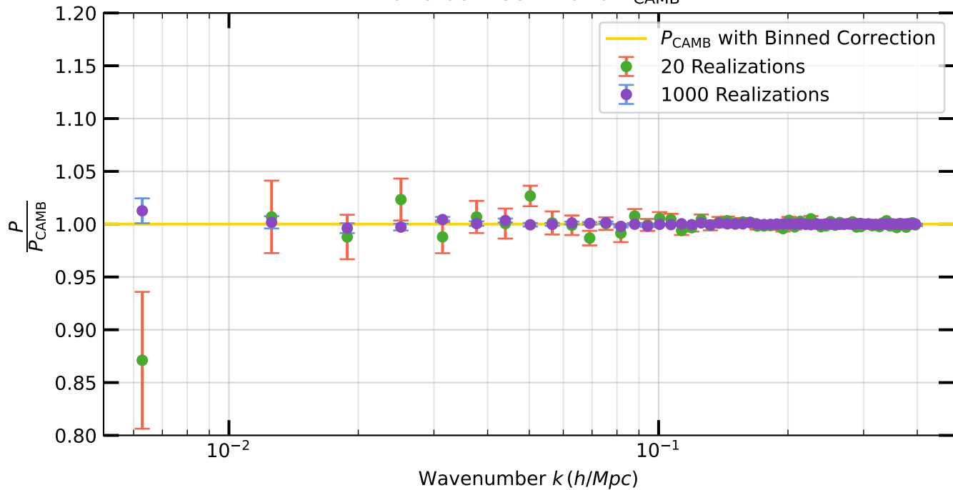
Ratio between P and P_{\text{CAMB}}
