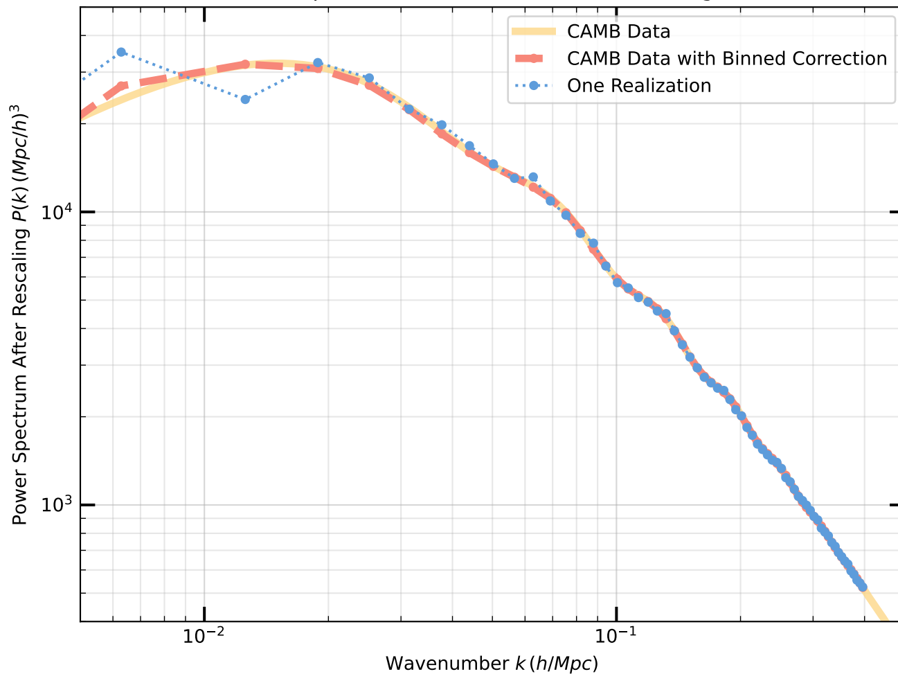
Power Spectrum Estimator with CAMB Using FFT
