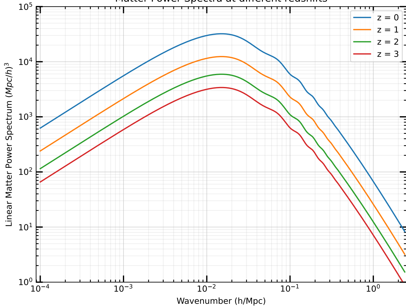
Matter Power Spectra at different redshifts
