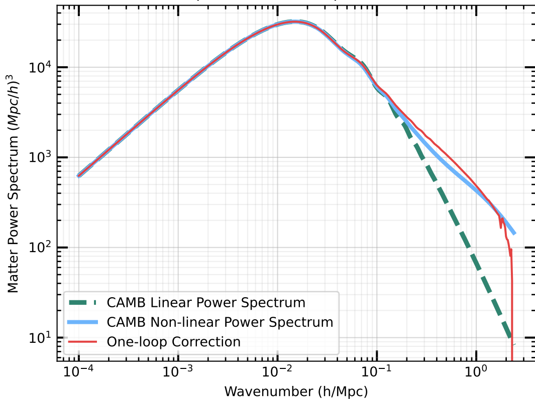
One-loop Matter Power Spectrum at z=0
