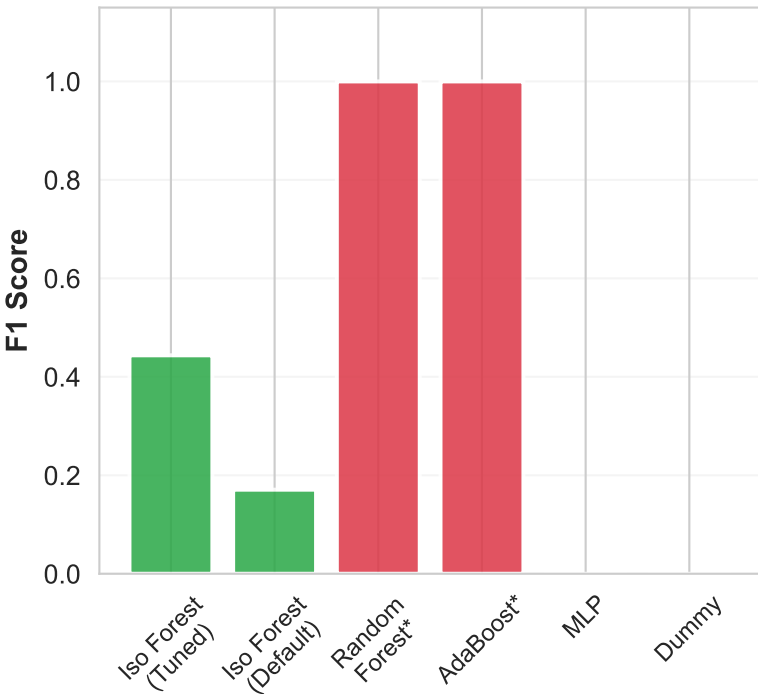
Model Comparison
