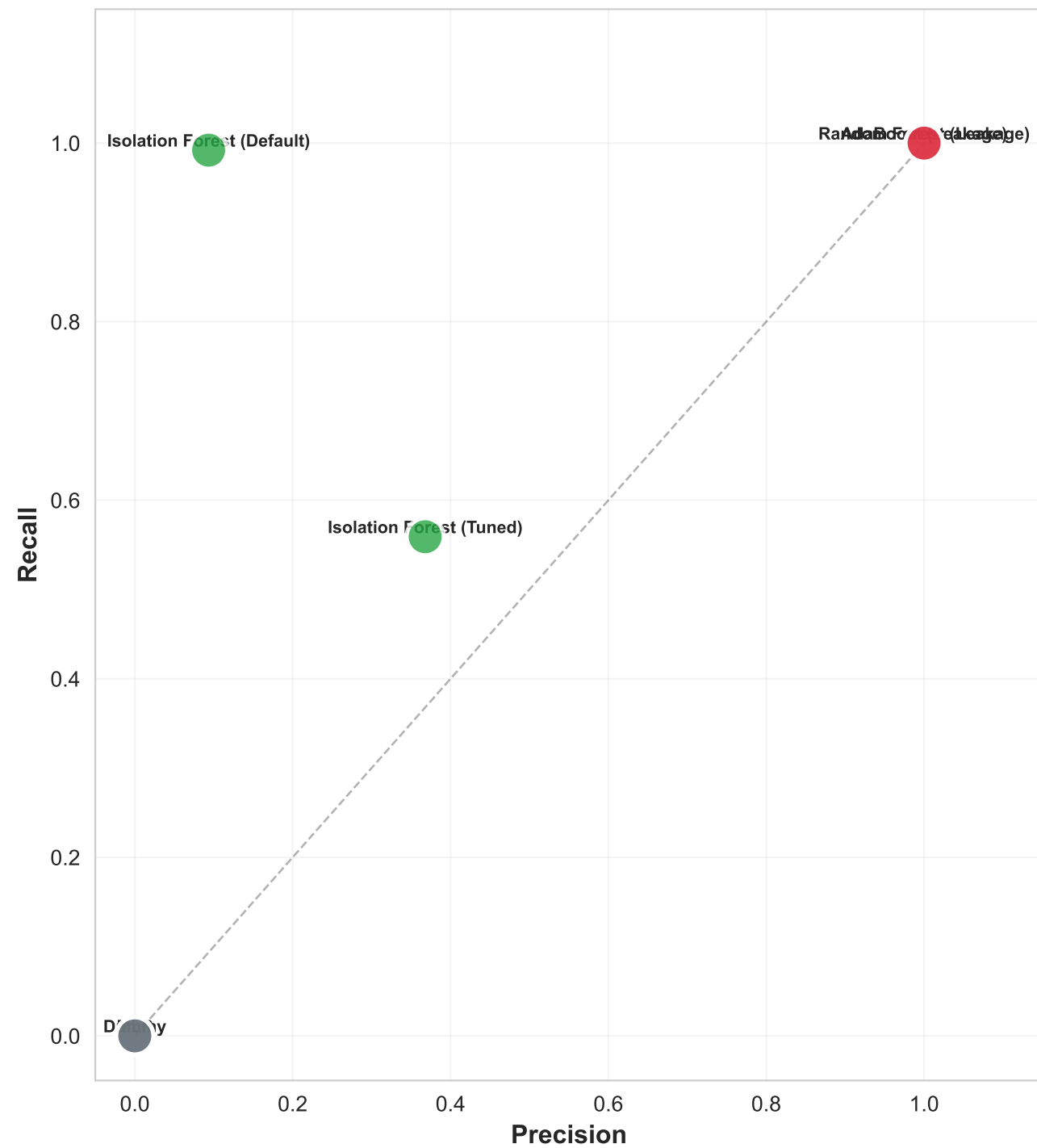
Precision vs Recall
