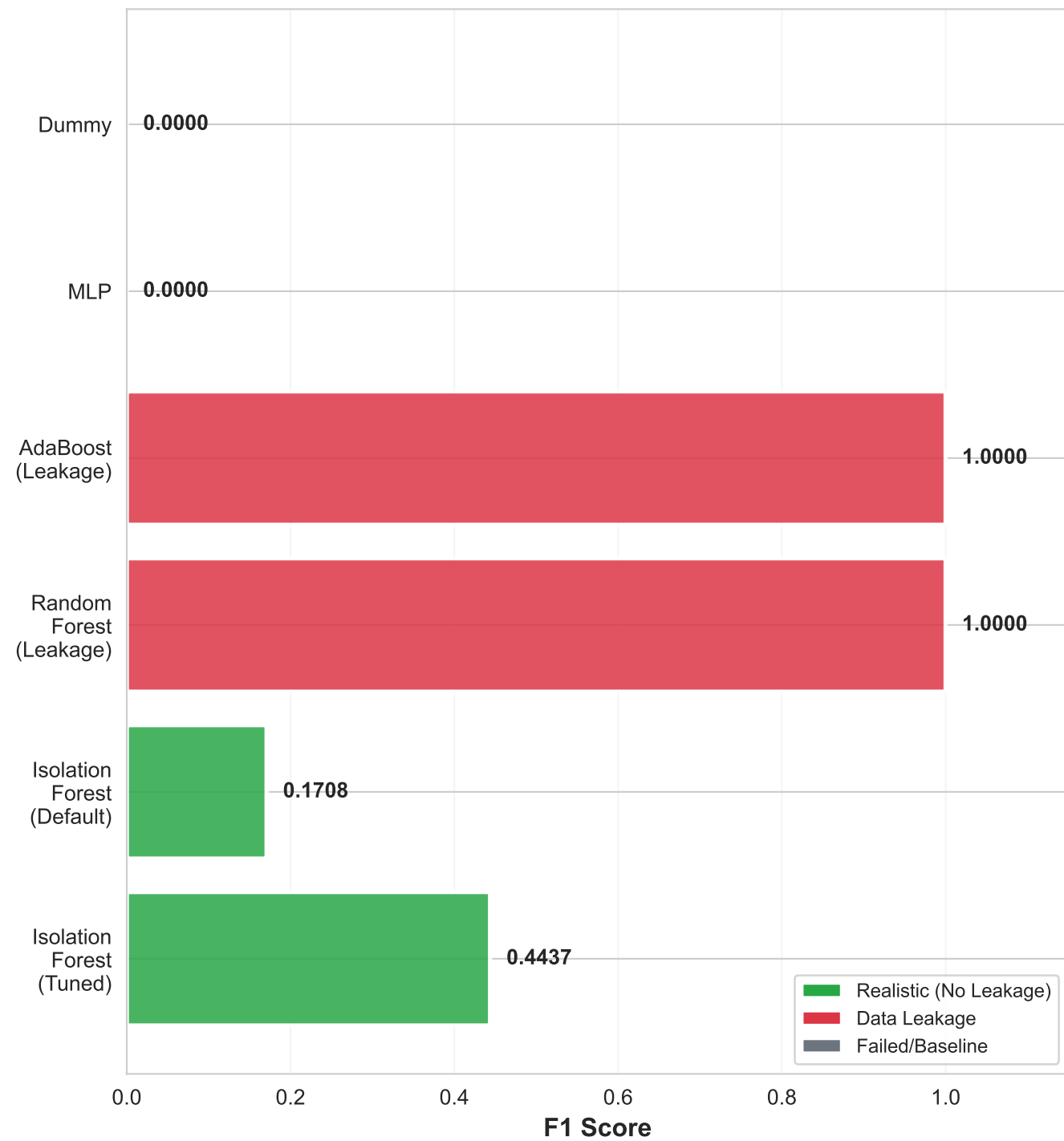
Model Comparison (Test Set)
