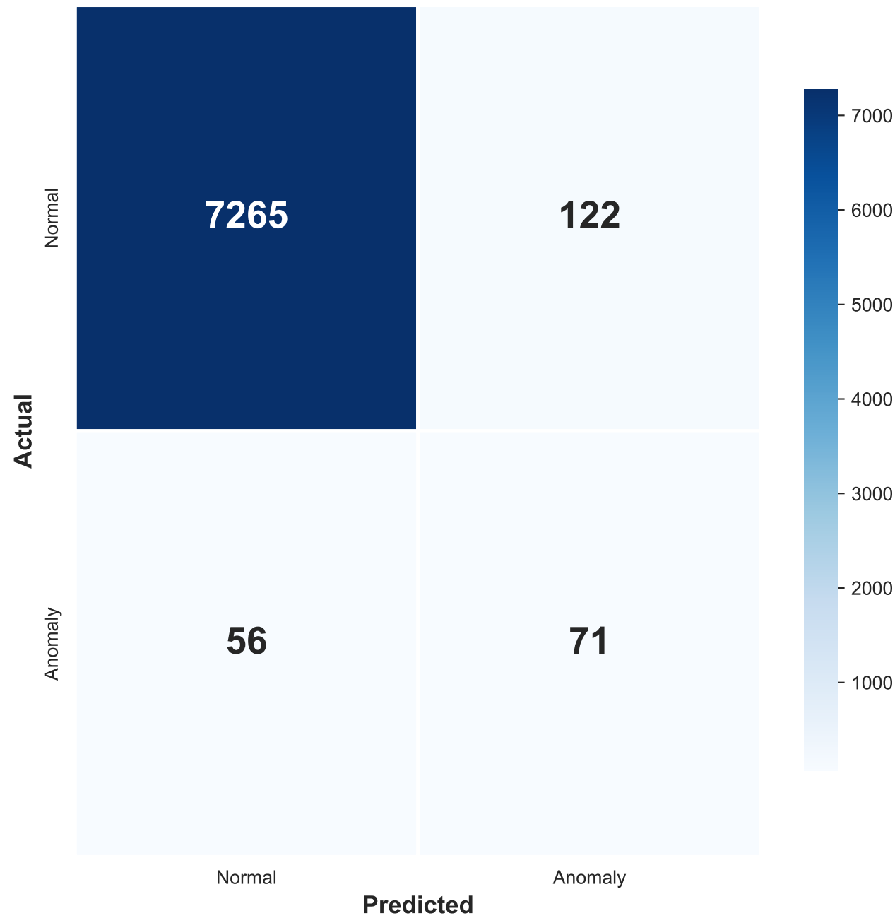
Confusion Matrix
