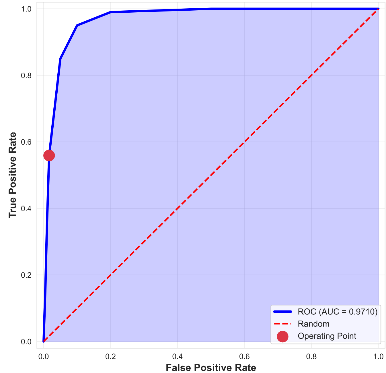
ROC Curve
