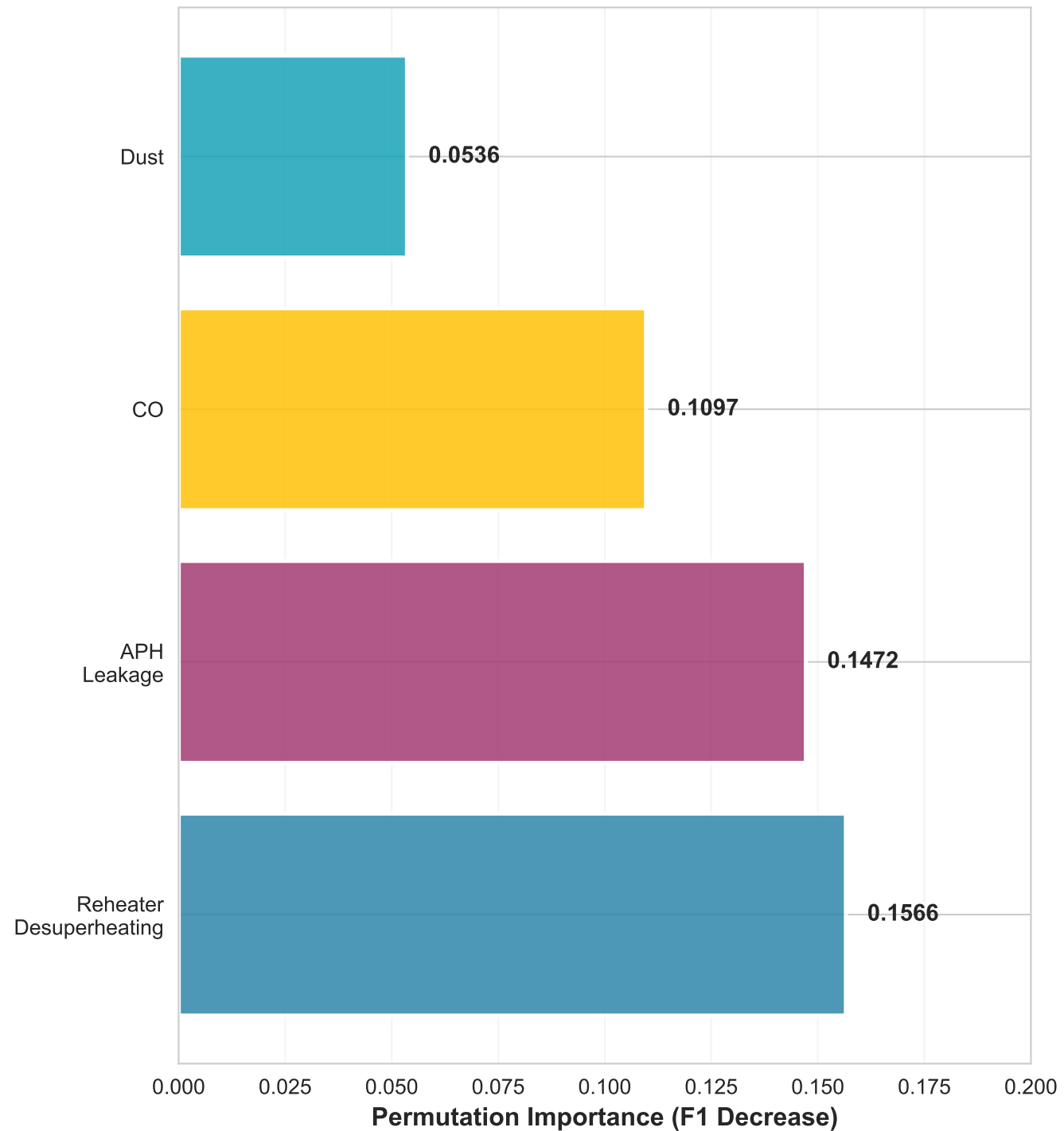
Permutation Importance
