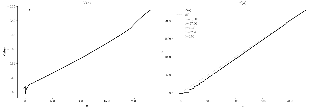
Figure 5: Infinite-horizon Problem
