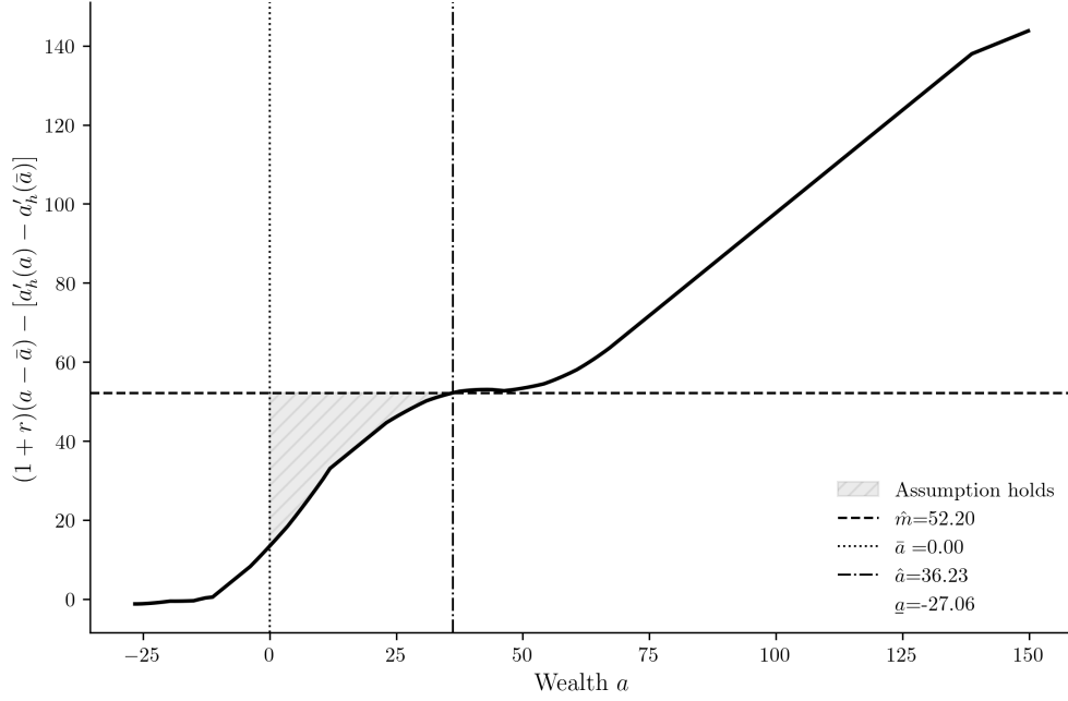
Figure 3: Assumption 7.1
