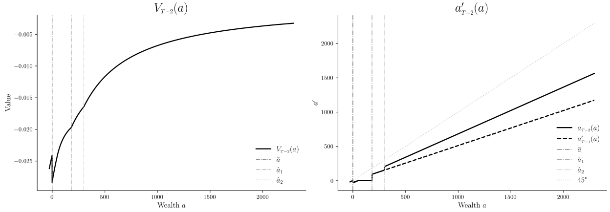
Figure 4: Two-period Problem
