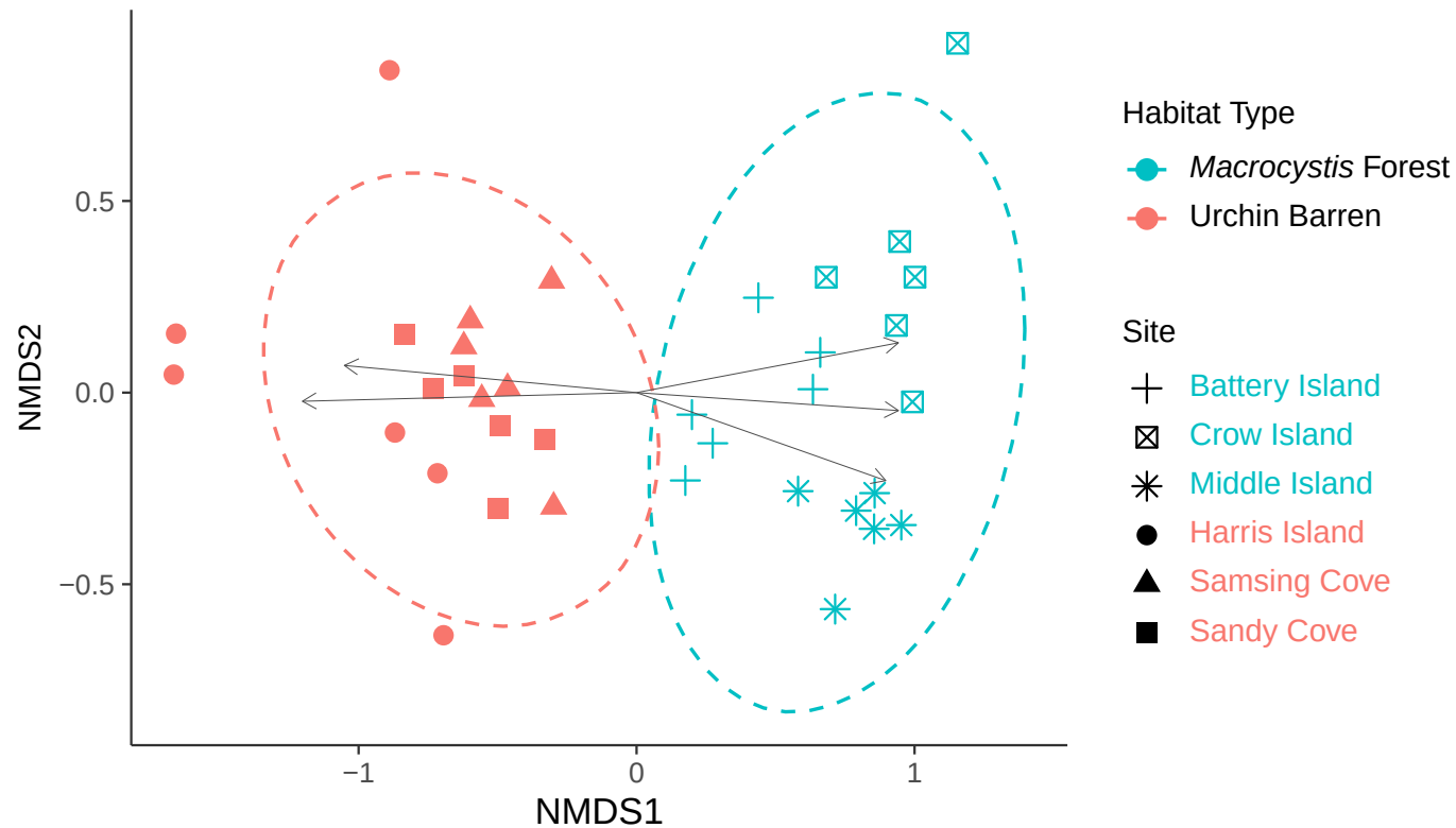
NMDS of community structure (stress = 0.114)
