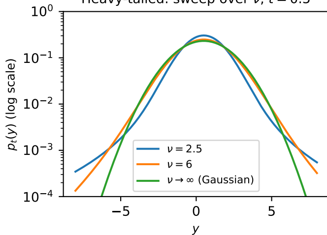
Heavy-tailed: sweep over \nu , t = 0.5
