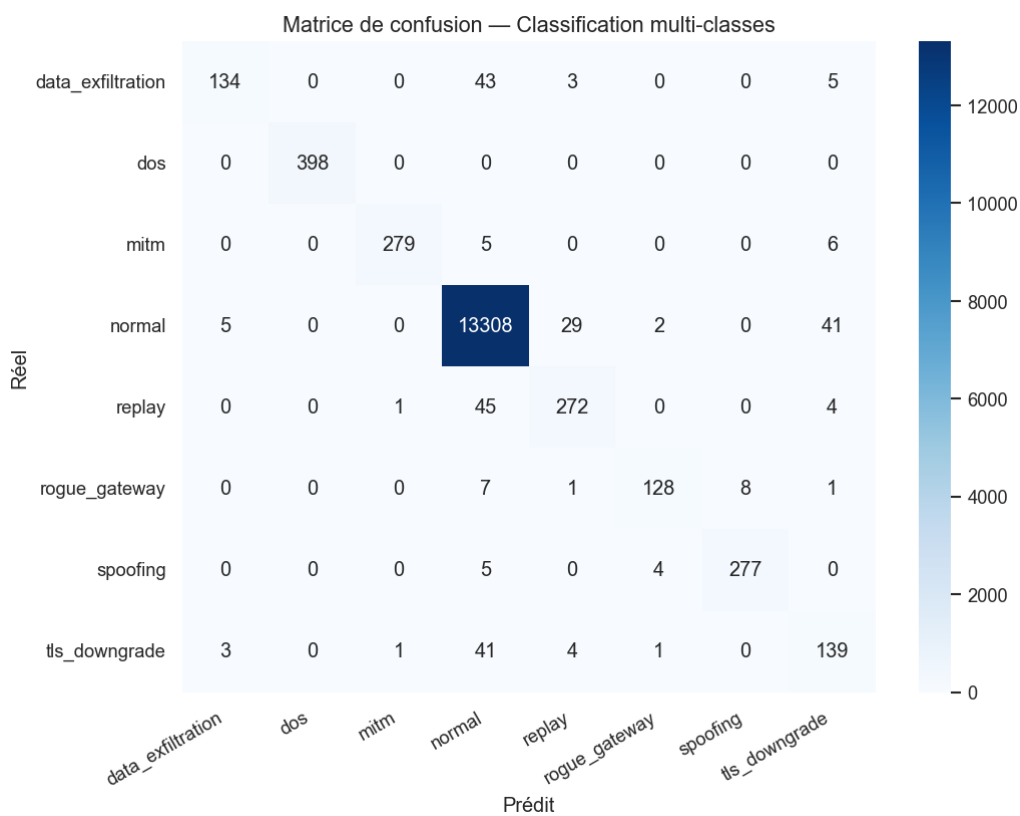
Fig. 5.11 : Random Forest – confusion multi-classes (8 classes)
