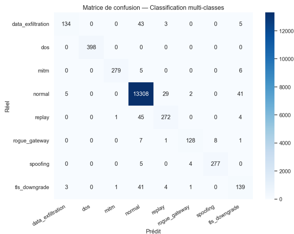
Fig. 5.8 : Random Forest – confusion multi-classes (8 classes)
