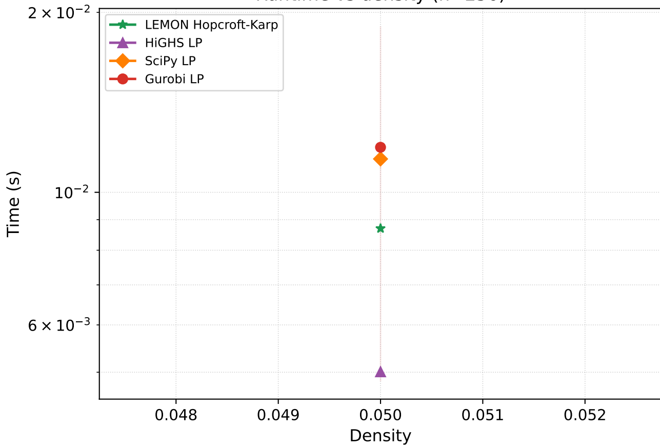
Runtime vs density (n=256)
