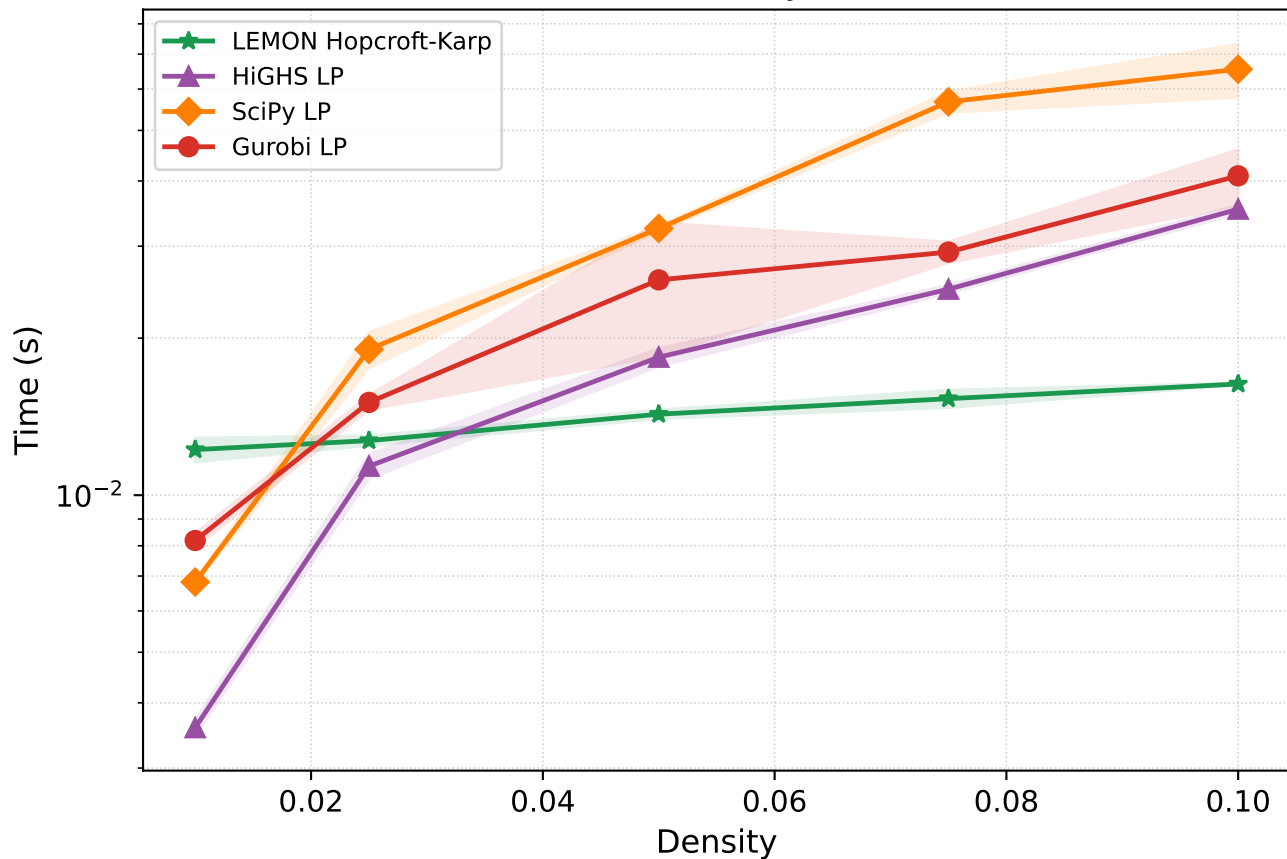
Runtime vs density (n=512)
