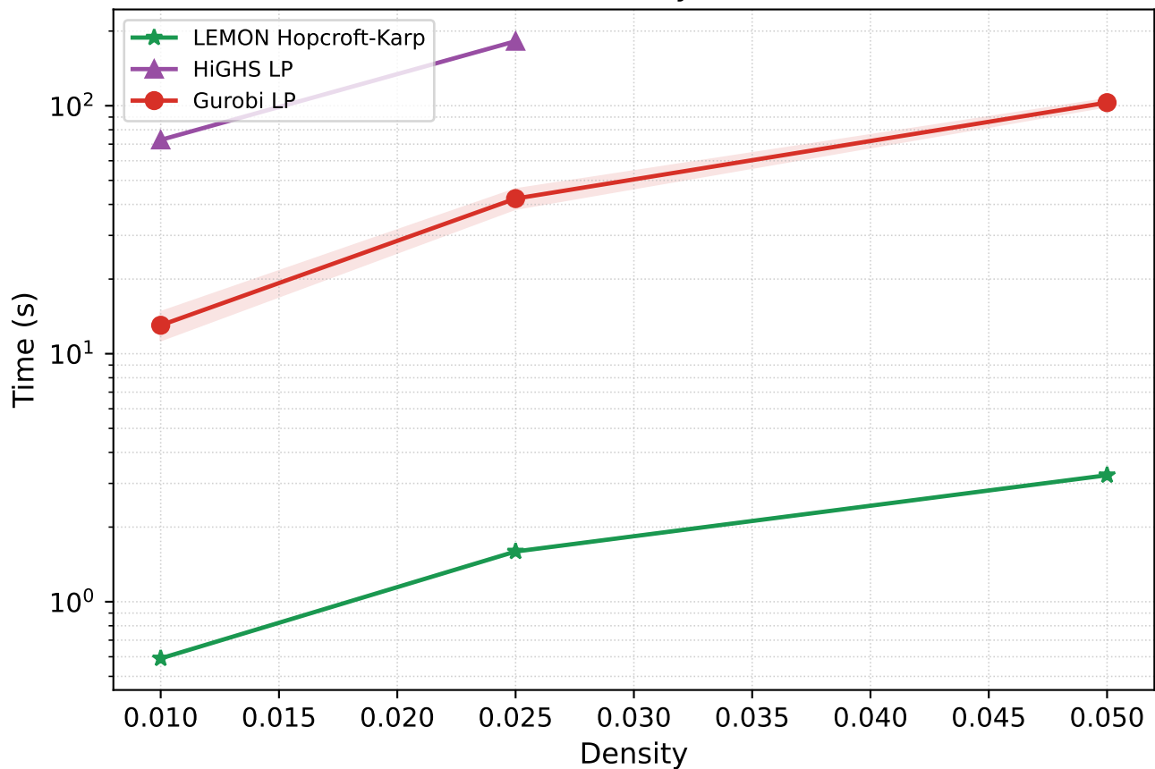
Runtime vs density (n=16384)
