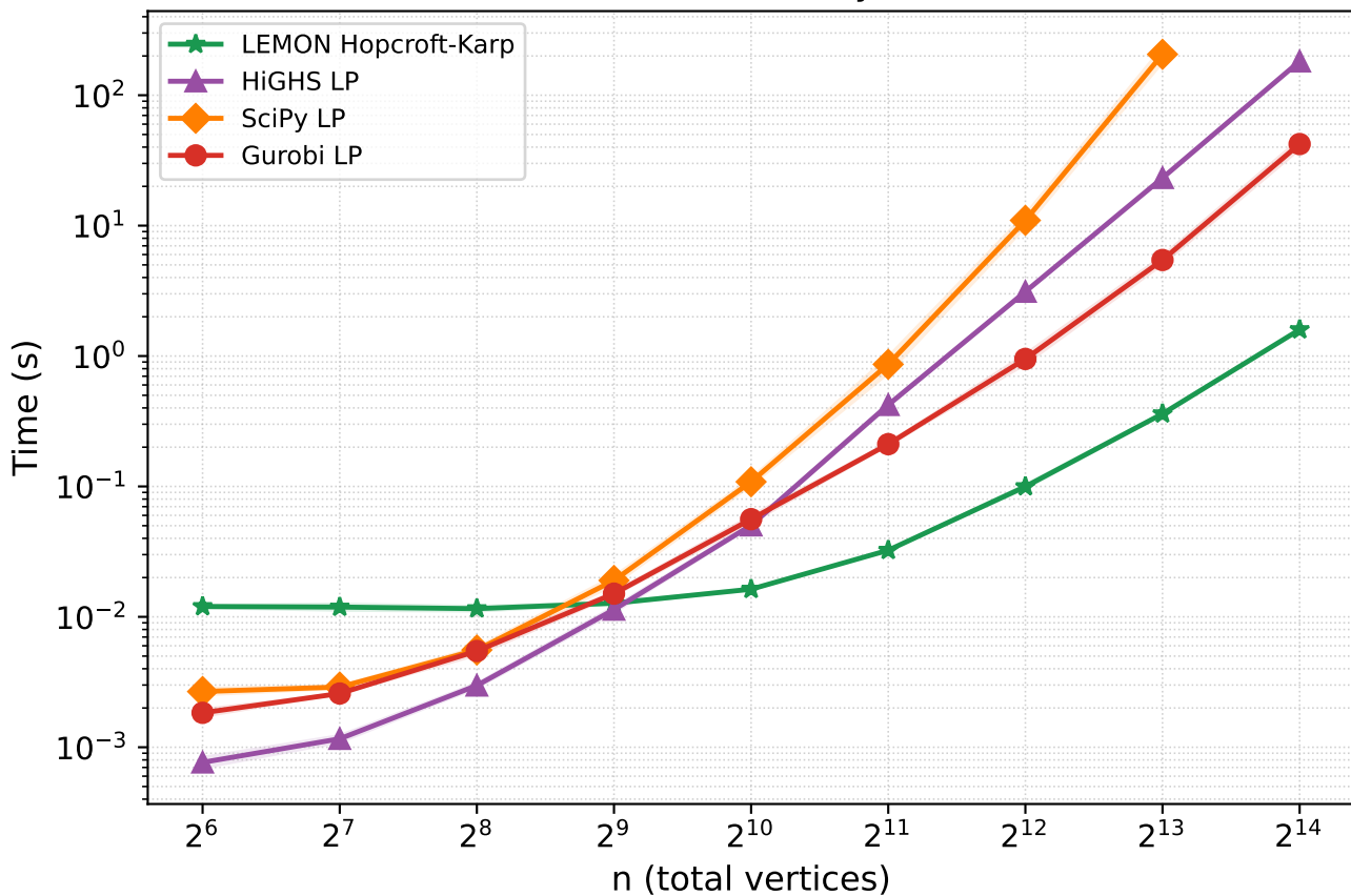
Runtime vs n (density=0.025)
