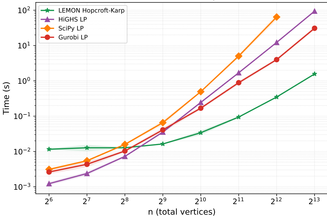
Runtime vs n (density=0.1)
