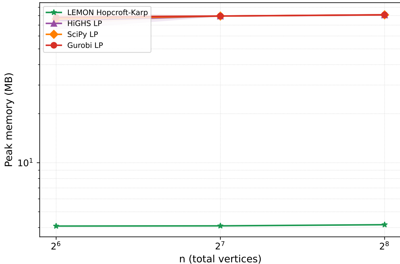
Memory vs n (density=0.05)
