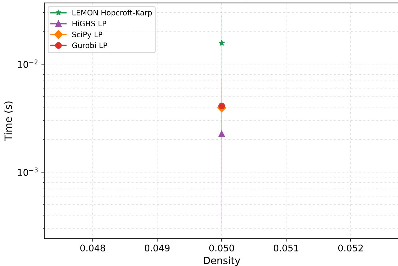
Runtime vs density (n=64)
