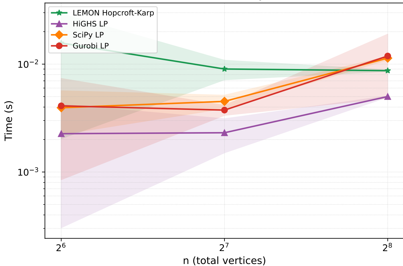
Runtime vs n (density=0.05)
