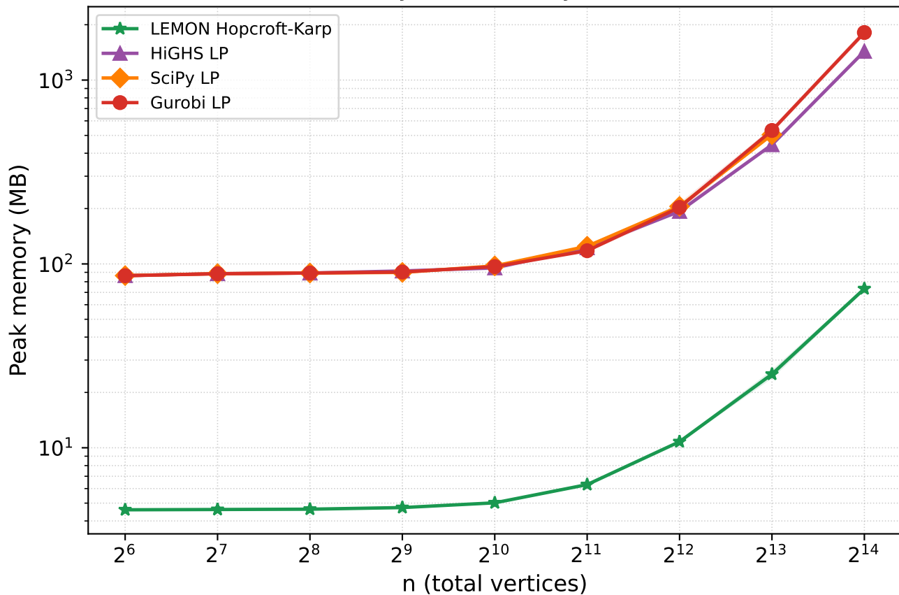
Memory vs n (density=0.025)
