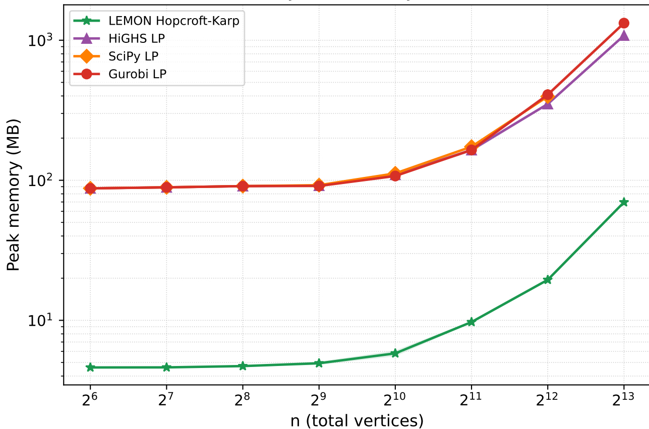
Memory vs n (density=0.075)
