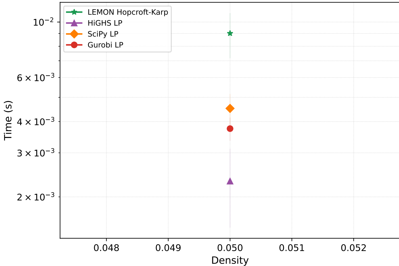
Runtime vs density (n=128)
